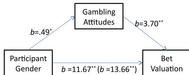
Figure 1: Mediation of gambling attitudes, Study 1. Results of gender difference in risk aversion for Study 2: total effects of gender on valuation b = 13.66 ( p < .01 ); direct effect b = 11.67 ( p < .01 ); indirect effect through mediator b = 1.80 ( p < .01 ).
