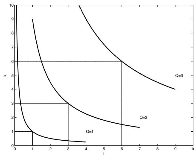
Figure 2: Isoquant Curves, Decreasing Returns to Scale.
