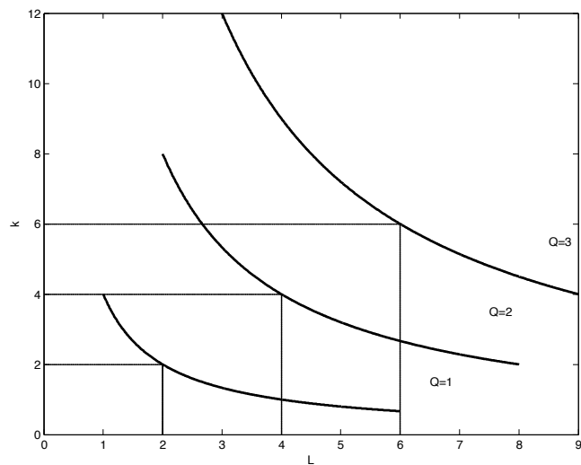
Figure 1: Isoquant Curves, Constant Returns to Scale.
