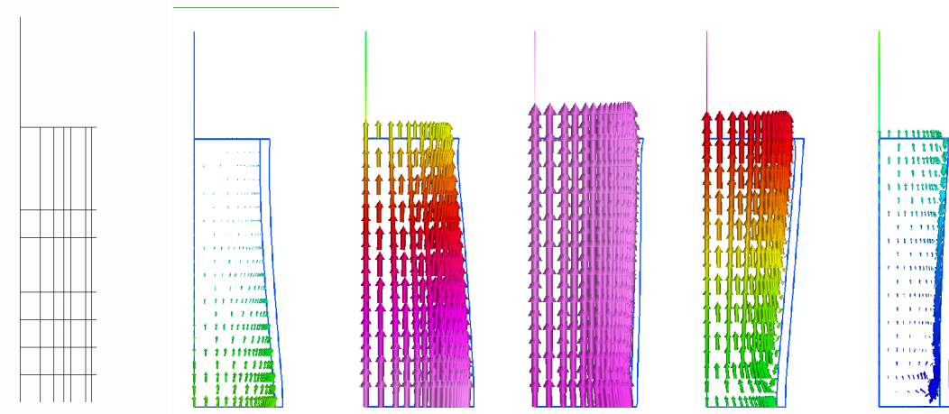
Figure 68.1: An example of the model results: pressure pulse propagation in a 2D axisymmetric model combined with an 1D model.
