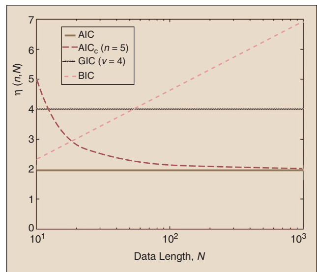
▲ 1. Penalty coefficients of AIC, GIC with \nu = 4 , \text{AIC}_c (for n = 5 ), and BIC as functions of the data length N .
