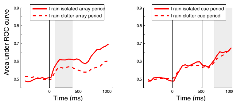
Fig. 2. Attention restores neural activity to a state that is similar to when the attended object is presented alone. Results are based on training a classifier with either 11 examples of isolated objects (solid lines) or with 11 examples of the same (attended) objects in cluttered displays (dashed line). The classifier was trained with either 300 ms of data from the array period ( Left , gray shaded region) before the attentional cue or 310 ms of data from the period following the onset of the attentional cue ( Right , gray shaded region). The classifier's performance was tested with either isolated-object trials (A) or with cluttered array data (B), using firing rates from 150 ms of data sampled in 50-ms sliding intervals. The results show that when training with data from the array period, better performance is achieved when training with isolated-object data compared with clutter data (left two plots), confirming that clutter reduces information about particular objects. Approximately equal levels of performance were obtained when training with either isolated or cluttered data from the period following the attentional cue (right two plots), indicating that attention caused the neural representation to enter a state that was similar to when objects were presented in isolation. It should be noted that for the isolated-object trials there is slightly more information about the stimuli when they are first shown, and hence the decoding accuracies are higher when training with data from the array period compared with training with data from the cue period (i.e., the solid blue trace in A Left is slightly higher than the solid blue trace in A Right ).
