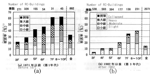
Fig.1 Statistics of damaged RC-buildings. (a) Old structures before 1971, and (b) Recent structures after 1982. (after Tohdo in AIJ, 1998)
