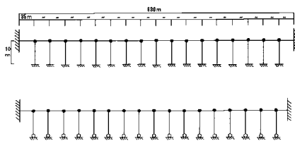
Fig.13 Structure model for Hanshin Highway
