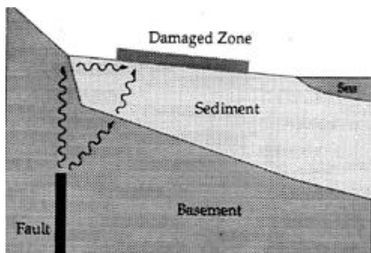
Fig.5 Concept to explain damaged belt zone with the underground topography (after Koketsu et al. in AIJ, 1996)
