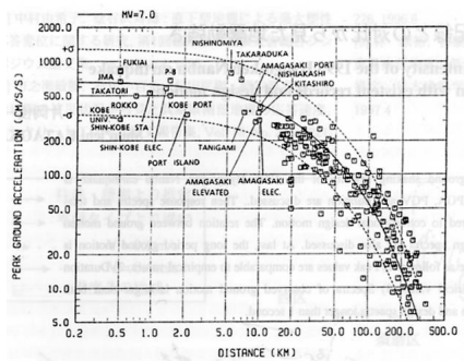
Fig.3 Attenuation of PGA during the 1995 Kobe earthquake (after Kataoka in AIJ, 1997)
