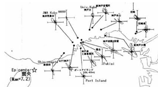
Fig.2 Observed strong motions (after Wakamatsu in AIJ, 1995)
