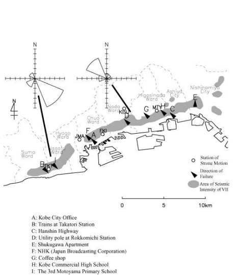
Fig.7 Direction of collapsed buildings and structures
