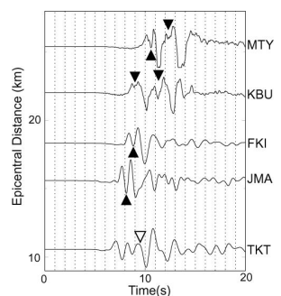
Fig.8 Velocity strong motions with effective phases contributed to the failure of buildings and structures
