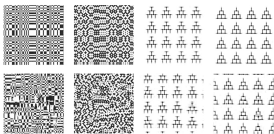
Figure 13. Synthesis of classic counterexamples to the Julesz conjecture (Julesz et al., 1978; Yellot, 1993) (see text). Top row: original artificial textures. Bottom row: Synthesized textures.
