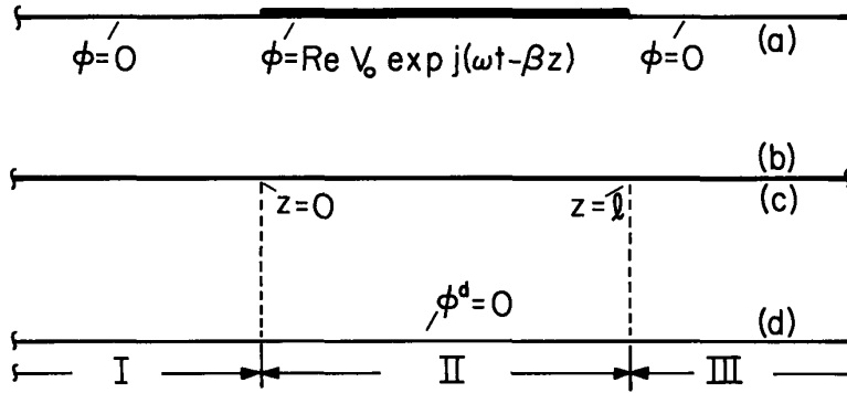
Fig. 5.17.3. A thin sheet moving with velocity U in the z direction enters the excitation region at z = 0 and leaves at z = \ell .
