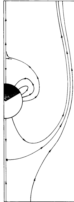
Fig. 5.5.5. Force lines in detail for regimes (e) for positive ions and (h) for negative ions. Here, all of the characteristic lines terminating on the particle also originate on the particle; hence, there is no charging. For the case shown, U = \pm 2bE , q = \pm q_c/2 .
