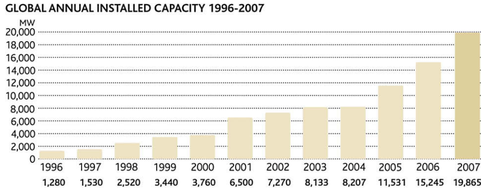
Fig. 1. Global annual installed wind power capacity (Source: Global Wind Energy Council, http://www.gwec.net/ , retrieved 9 September 2008.)
