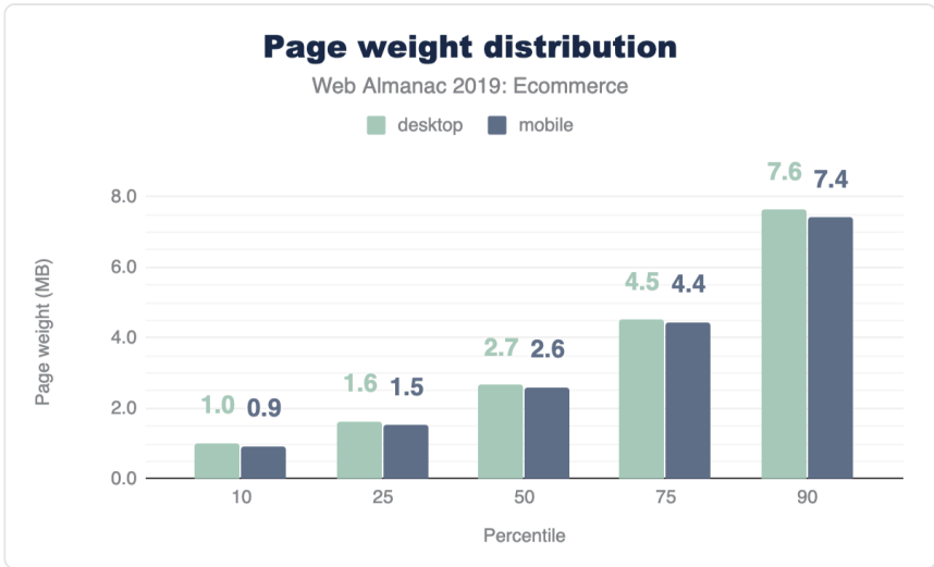
Figure 13.7. Distribution of ecommerce page weight.
