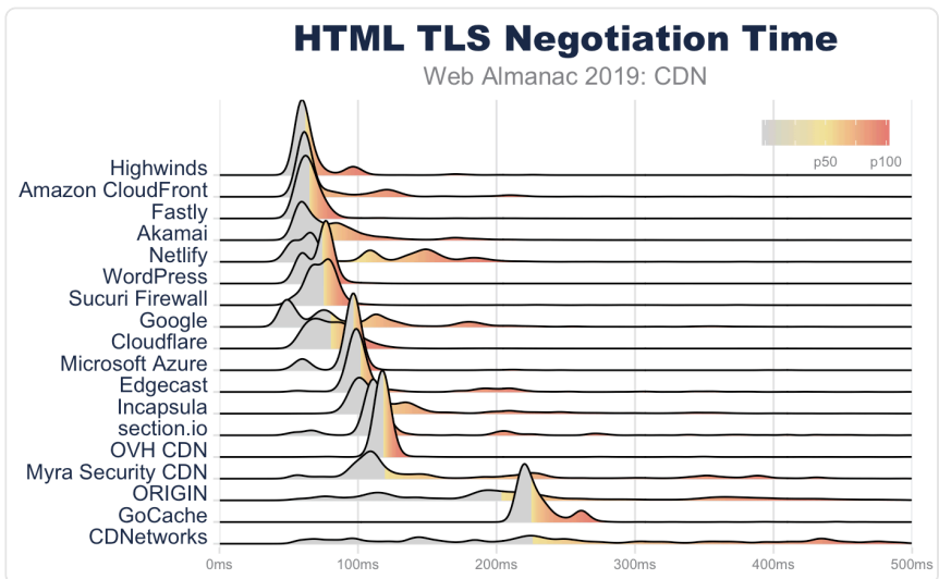
Figure 17.8. HTML TLS negotiation time.
