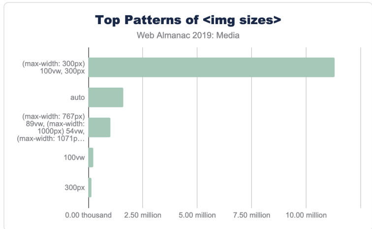
Figure 4.16. Top patterns of <img sizes> .
