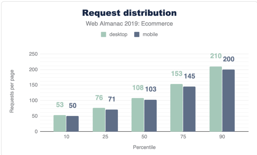
Figure 13.8. Distribution of requests per ecommerce page.
