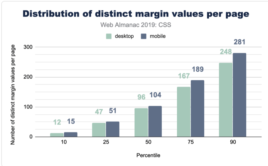
Figure 2.18. Distribution of the number of distinct margin values per page.
