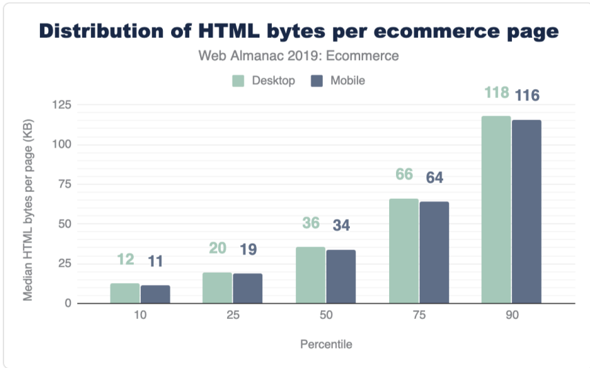
Figure 13.11. Distribution of HTML bytes (in KB) per ecommerce page.
