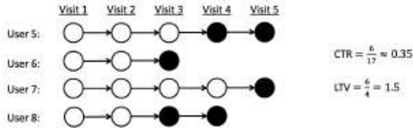
Figure 16.8: Click through rate (CTR) versus life-time value (LTV). Each circle represents a user visit; black circles are visits at which the user clicks. Adapted from Theocharous et al. (2015).
