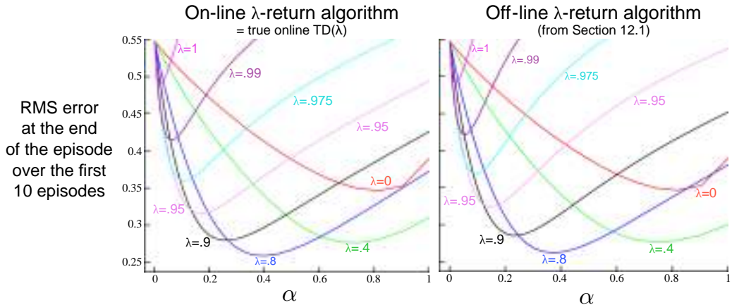
Figure 12.8: 19-state Random walk results (Example 7.1): Performance of online and off-line \lambda -return algorithms. The performance measure here is the VE at the end of the episode, which should be the best case for the off-line algorithm. Nevertheless, the online algorithm performs subtly better. For comparison, the \lambda=0 line is the same for both methods.
