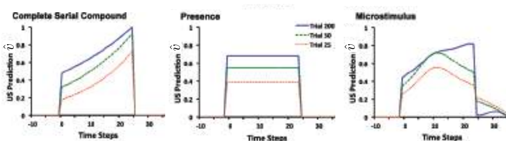
Figure 14.4: Time course of US prediction over the course of acquisition for the TD model with three different stimulus representations. Left: With the complete serial compound (CSC), the US prediction increases exponentially through the interval, peaking at the time of the US. At asymptote (trial 200), the US prediction peaks at the US intensity (1 in these simulations). Middle: With the presence representation, the US prediction converges to an almost constant level. This constant level is determined by the US intensity and the length of the CS–US interval. Right: With the microstimulus representation, at asymptote, the TD model approximates the exponentially increasing time course depicted with the CSC through a linear combination of the different microstimuli. Adapted with minor changes from Learning & Behavior , Evaluating the TD Model of Classical Conditioning, volume 40, 2012, E. A. Ludvig, R. S. Sutton, E. J. Kehoe. With permission of Springer.
