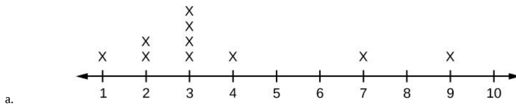
Figure 2.19 Terry's distribution has a right (positive) skew.
