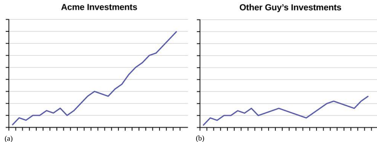
Figure 1.14 As the graphs show, Acme consistently outperforms the Other Guys!
