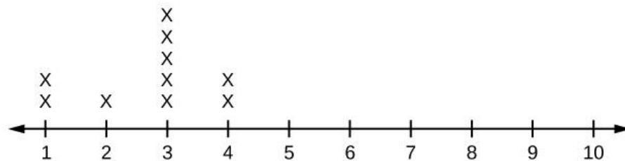
Figure 2.20 Davi's distribution has a left (negative) skew.
