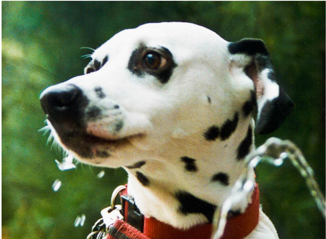
Figure 9.1 You can use a hypothesis test to decide if a dog breeder's claim that every Dalmatian has 35 spots is statistically sound. (Credit: Robert Neff)
